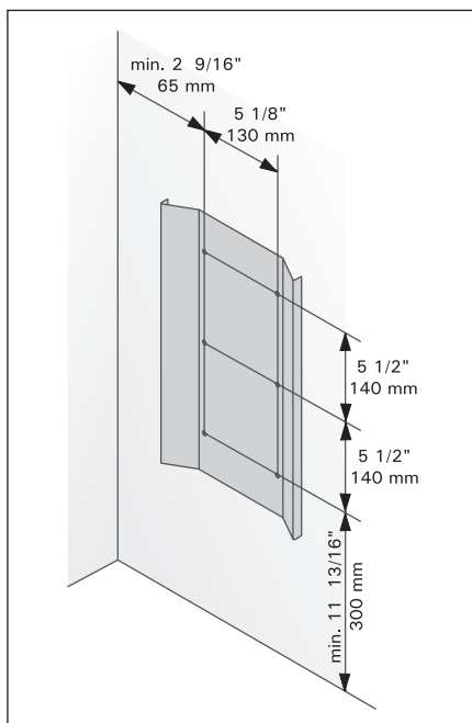
Figure 6. Location of the mounting rack of the heater
