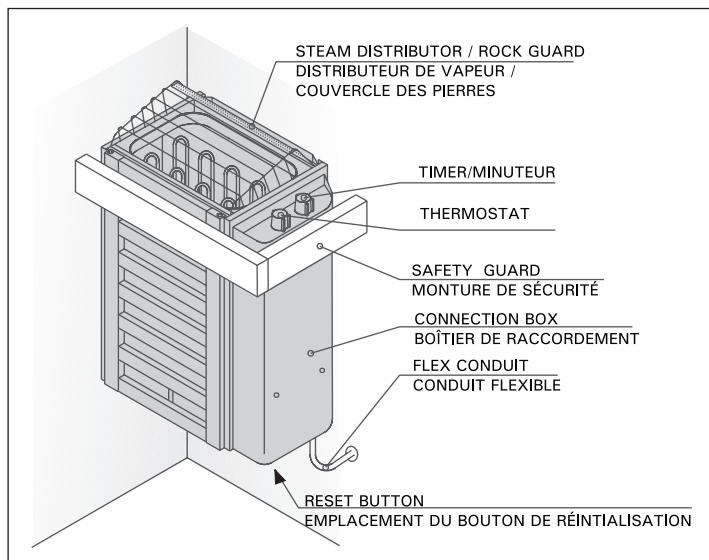
Figure 9. Connections and parts of the heater
