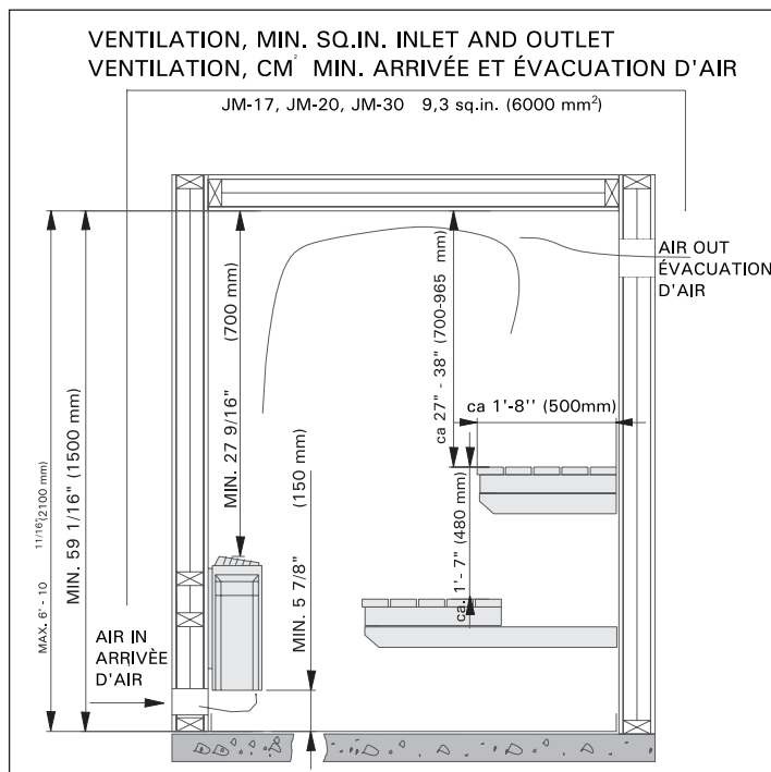
Figure 4. Sauna room Figure 4. Sauna
